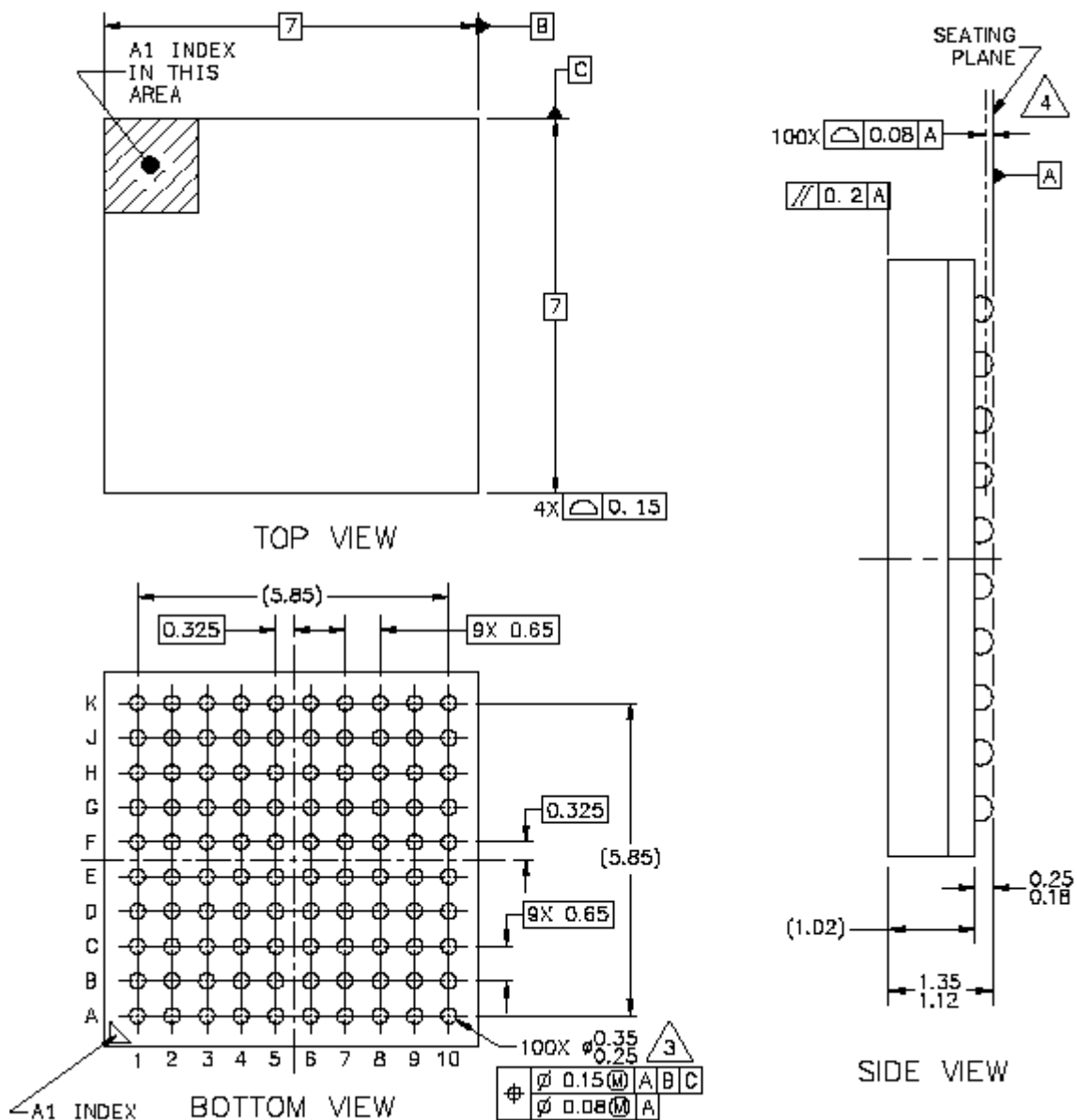
Figure 5. 100 MAPBGA Package Diagram 7 x 7 x 1.35 mm
