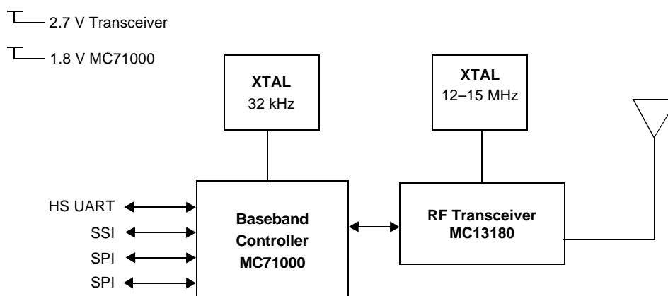
Figure 2. Sample Two-Chip Bluetooth Solution
