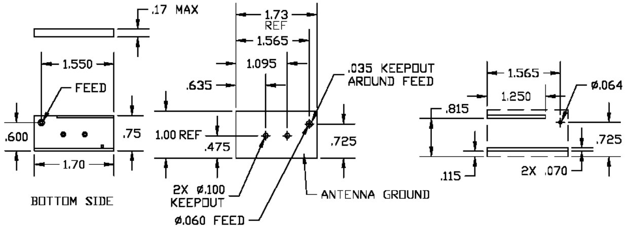
Part Dimensions
