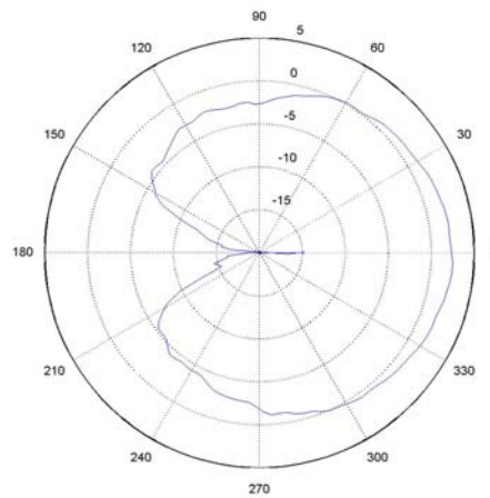
Gain at 2500 MHz Phi = 90 degrees
